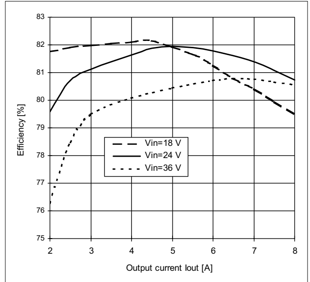
Efficiency (typ.)
